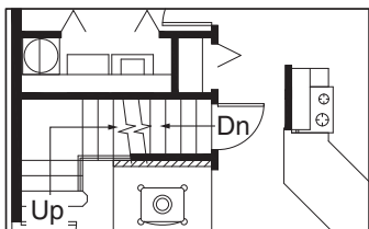
Alternate Basement Stairs
